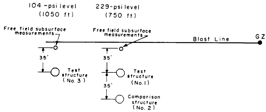
Fig. 1—Structure locations.
